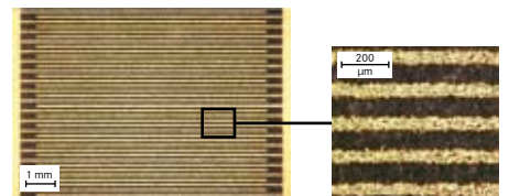
Sensor structure on LCP Vectra E820i-LDS, lines and spaces: 75 µm/75 µm.
